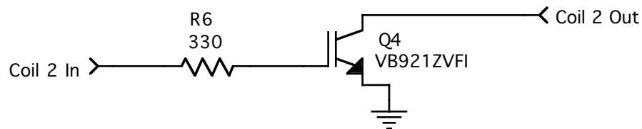
Ignition Coil Driver 2
