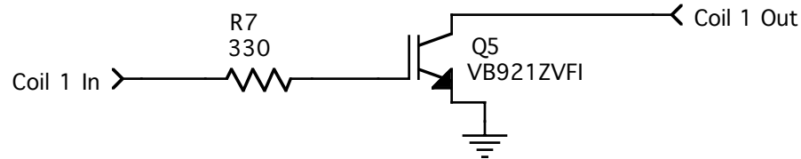
Ignition Coil Driver 1
